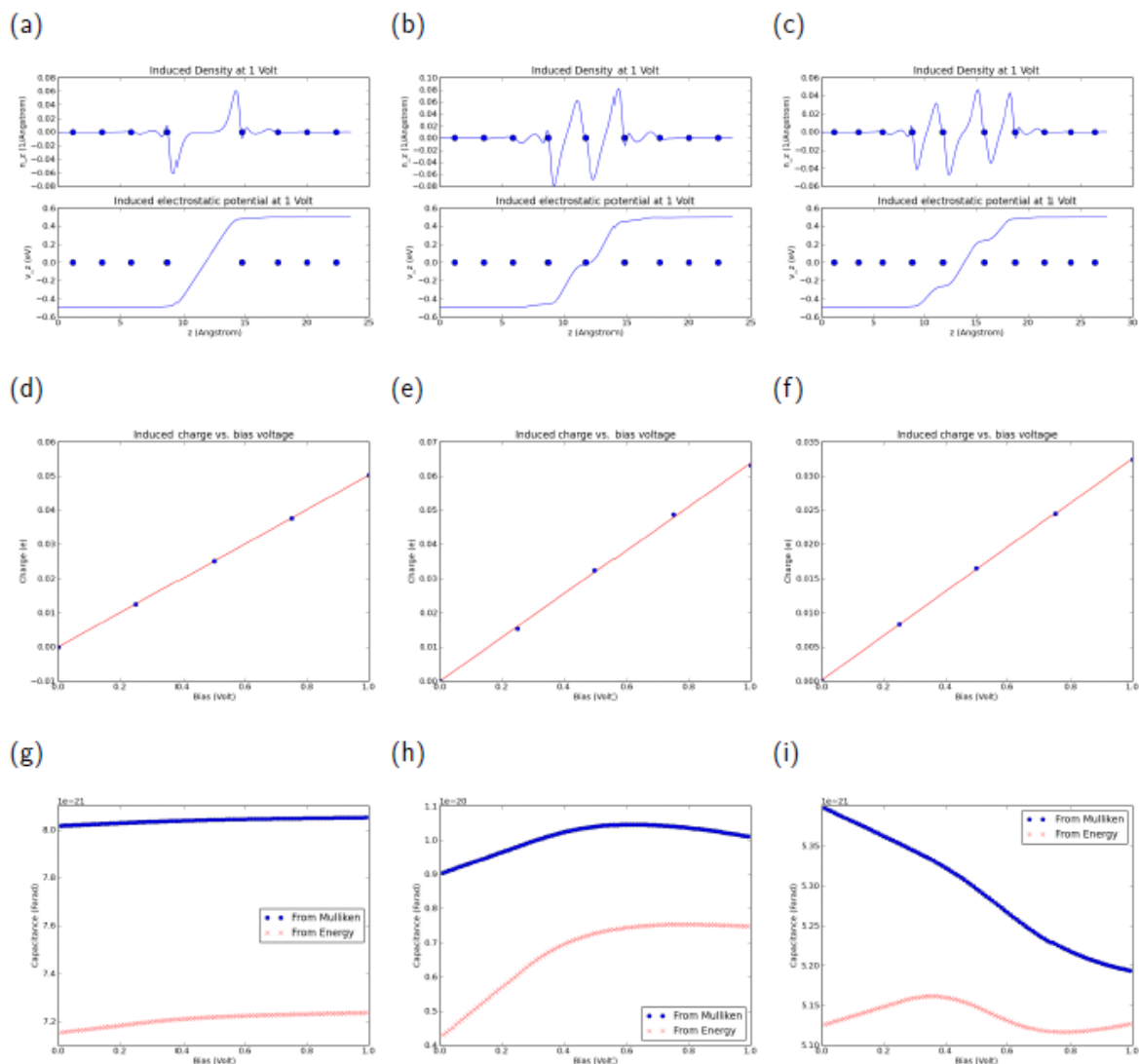
Figure III-2 (a-c) Induced charge densities and induced electrostatic potentials. (d-f) Variation of charge accumulation at electrodes with respect to applied voltage differences (g-i) Obtained capacitances with varying potentials.
