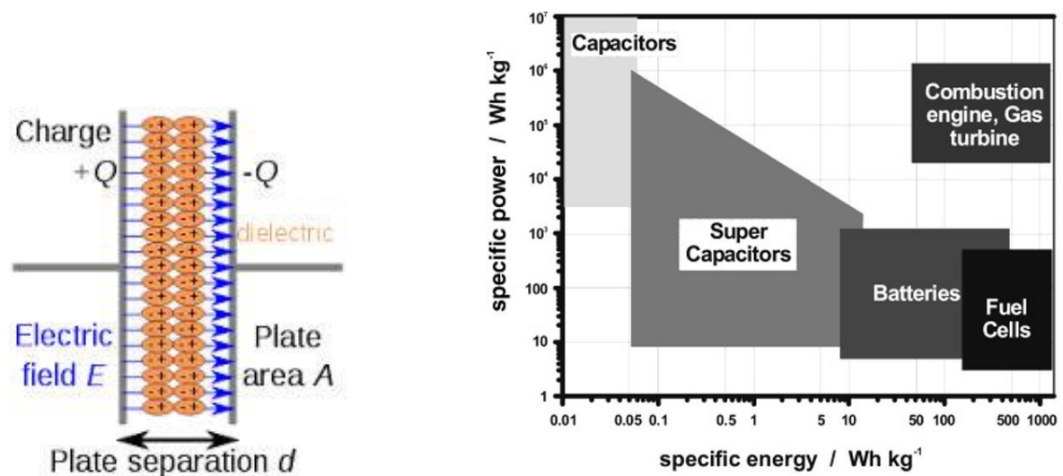
Figure III-1 (a) Schematics of double layer capacitor. (b) Ragone graphics of various energy storage systems [14].
